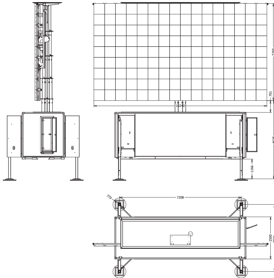
Technical Drawing
