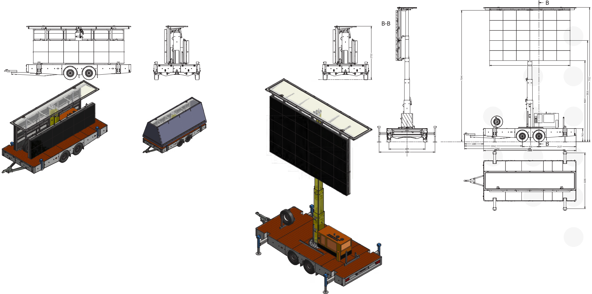
Technical Drawing
